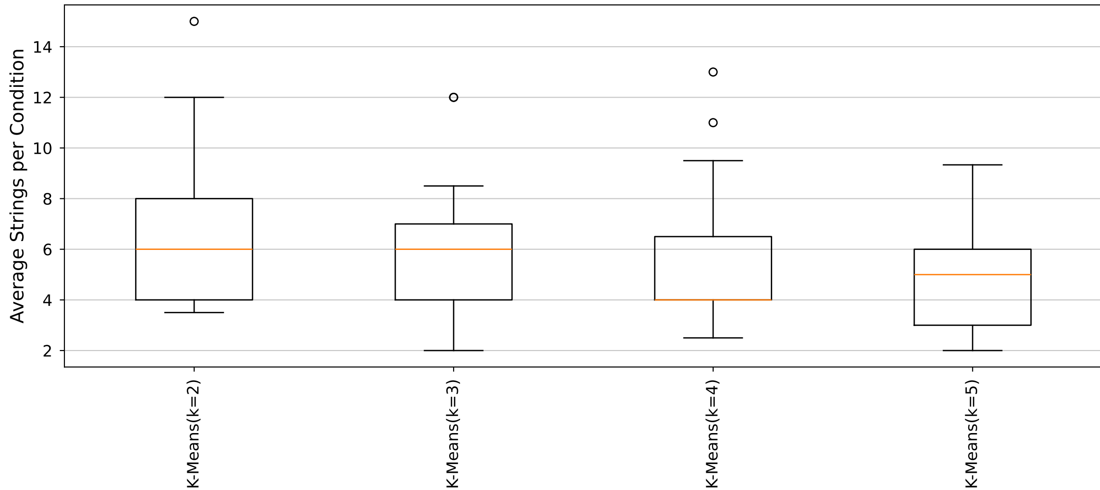
YARA Rules Average Strings per Condition Distribution (Cluster37_Size5 dataset)
